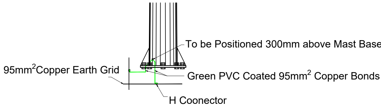
Monopole Base Plate to Earth Grid
