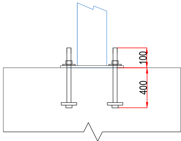
COLUMN BASE CONNECTION ( FOR REFERENCE ONLY)
