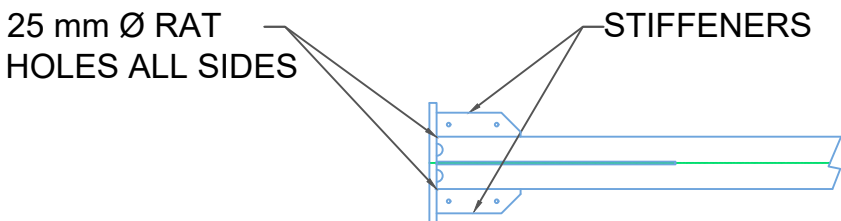
VIEW B-B
